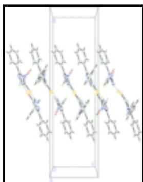
Fig. 2. The crystal packing of the title compound, viewed along the b axis. Hydrogen bonds are shown as dashed lines.
